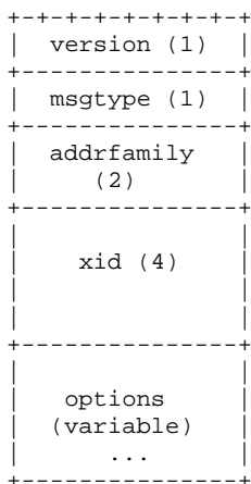
Figure 1: Format of a MADCAP message
