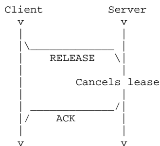
Figure 5: Timeline diagram of messages exchanged in Address Release example
