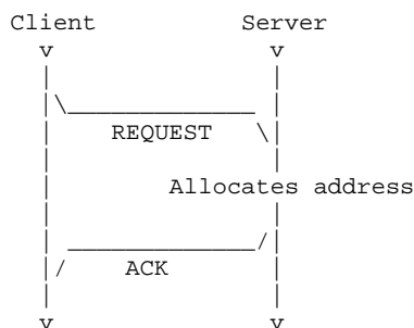
Figure 6: Timeline diagram of messages exchanged in Unicast Address Allocation example
