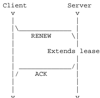
Figure 4: Timeline diagram of messages exchanged in Lease Extension example
